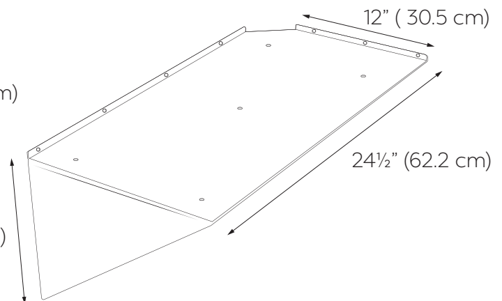
Stainless Still Mounting Bracket
