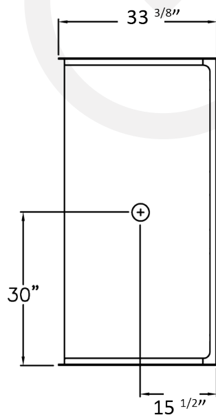
TOP VIEW
