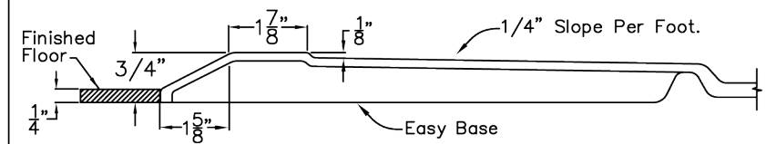
Detail of 3/4" Threshold
