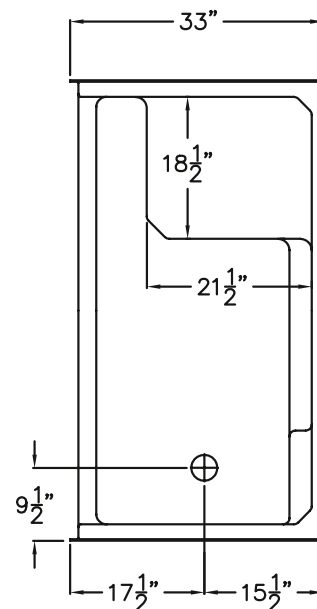
TOP VIEW
