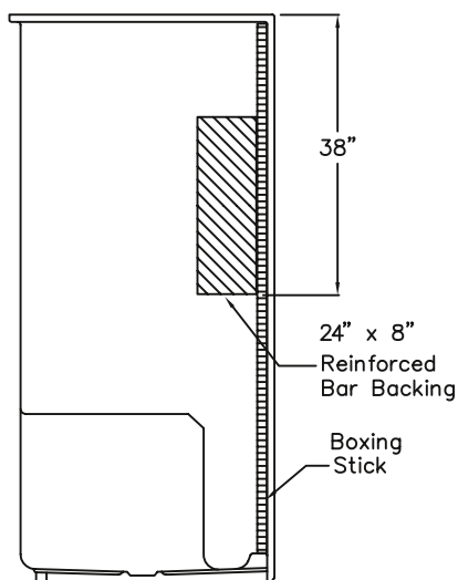
SEAT SIDE VIEW
